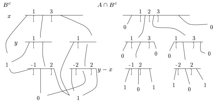
Figure 11: Testing for inclusion
