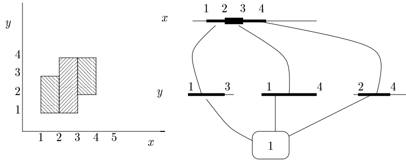
Figure 2: Enforcing Disjointness
