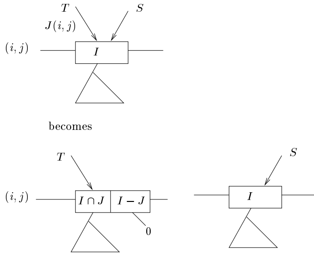
Figure 8: Tightening Intervals
