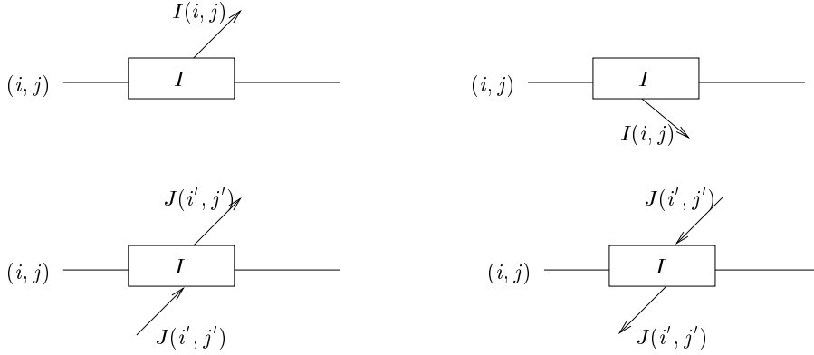
Figure 7: Simple Propagation
